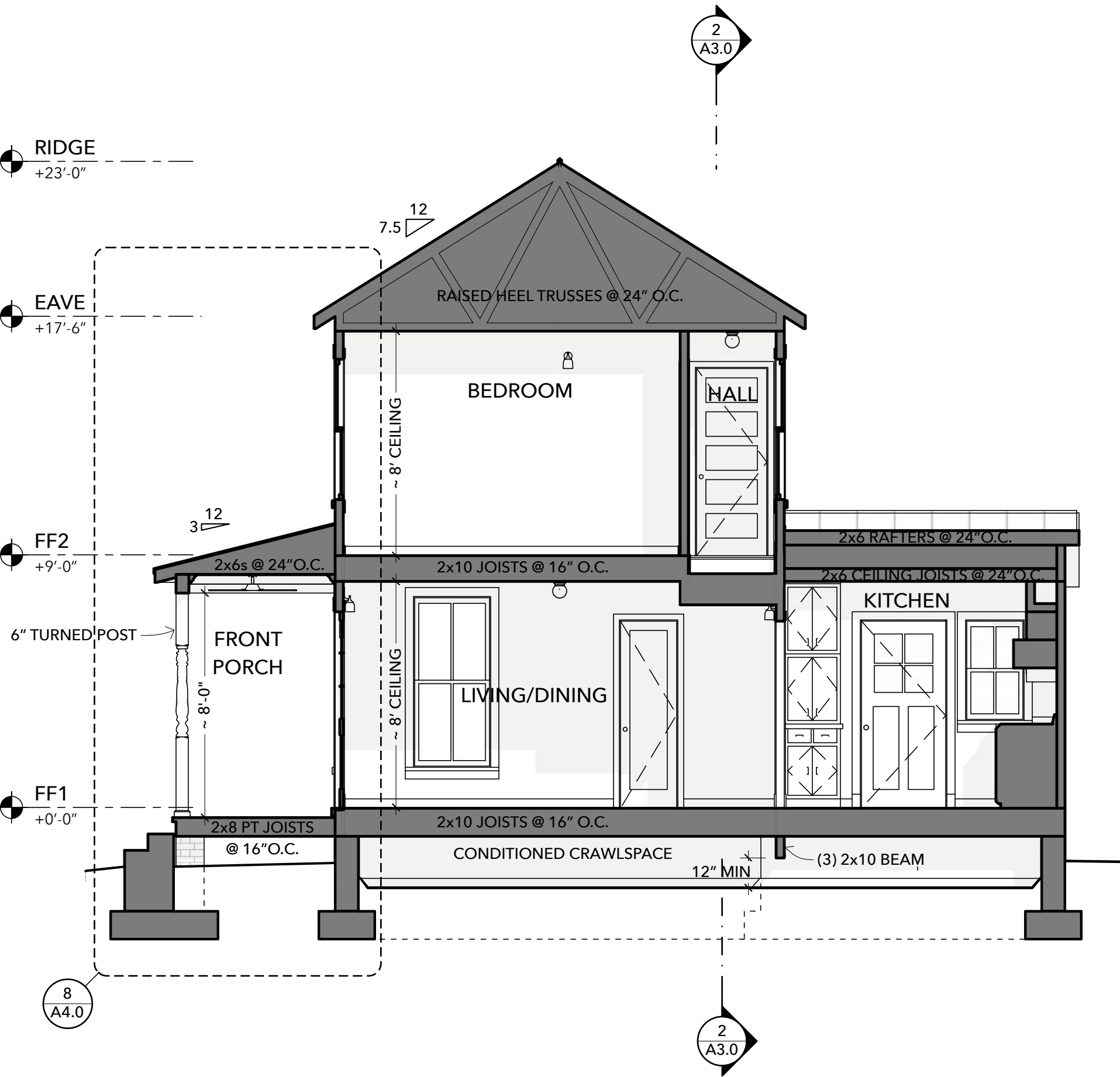
1 TRANSVERSE SECTION SCALE: 1/4" = 1'-0"
