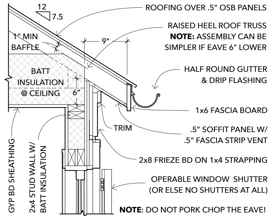
2 MAIN ROOF EAVE DETAIL SCALE: 1" = 1'-0"
