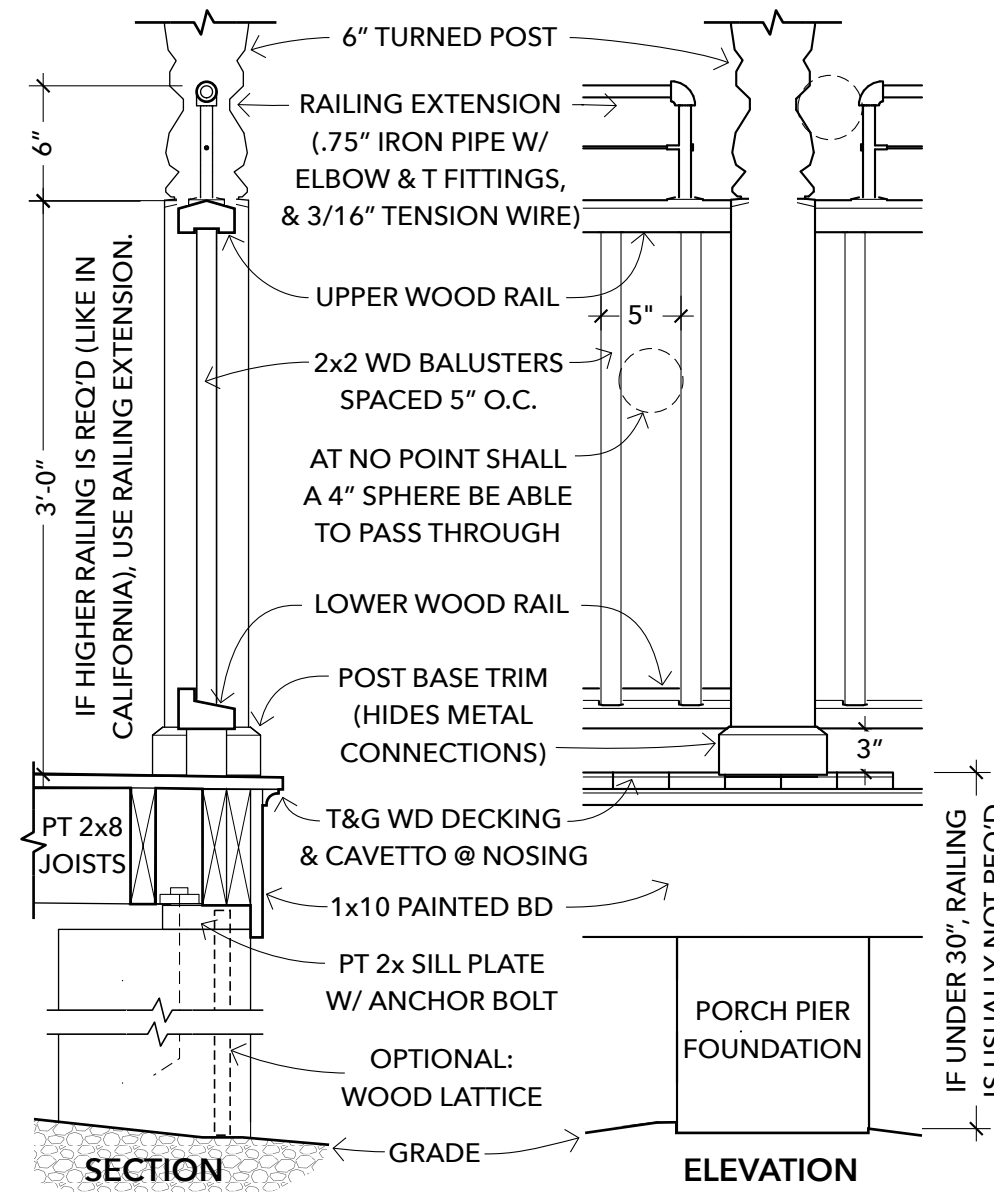
5 PORCH (SHOWS RAILING OPTIONS) SCALE: 1" = 1'-0" IF 42\"/>
