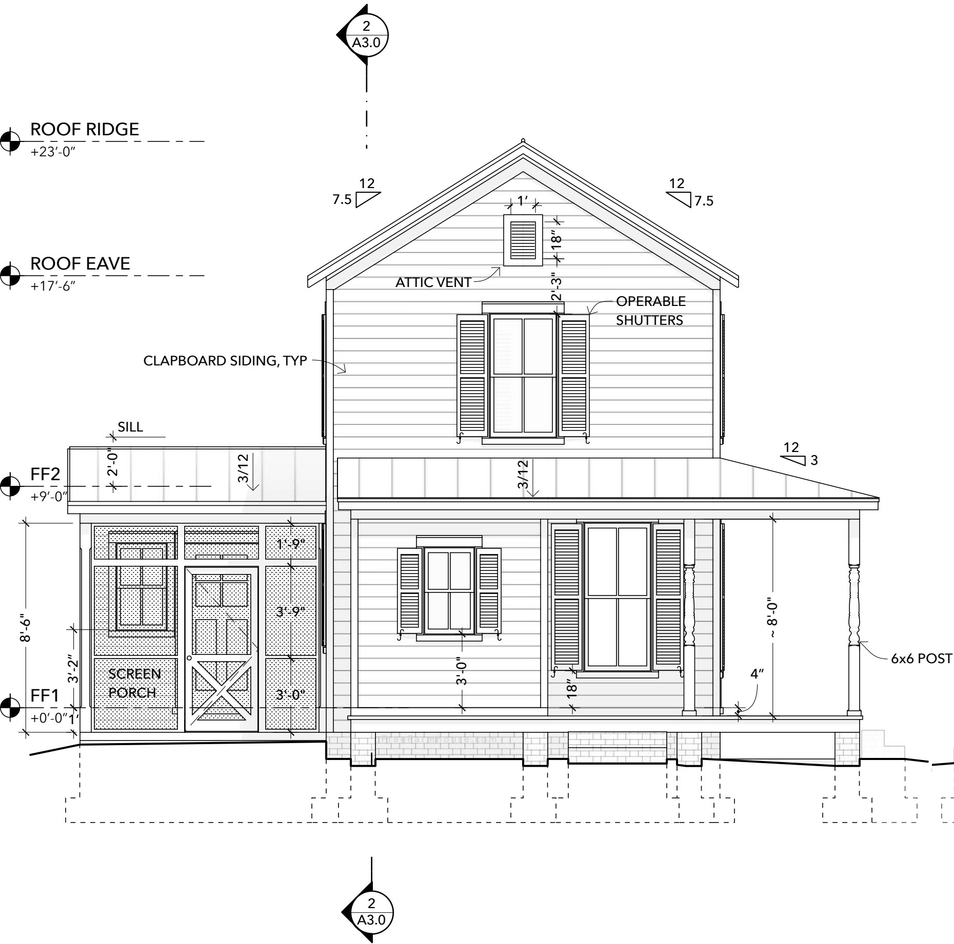
1 WEST ELEVATION SCALE: 1/4" = 1'-0"
