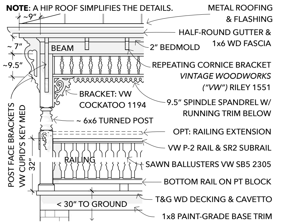
9 PORCH ORNAMENT (OPTION) SCALE: 1/2" = 1'-0" GINGERBREAD DECORATIONS
