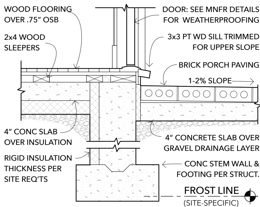
1C FOUNDATION OPTION C: SLAB SCALE: 1" = 1'-0" UNCOMMON FOR OLD HOUSES
