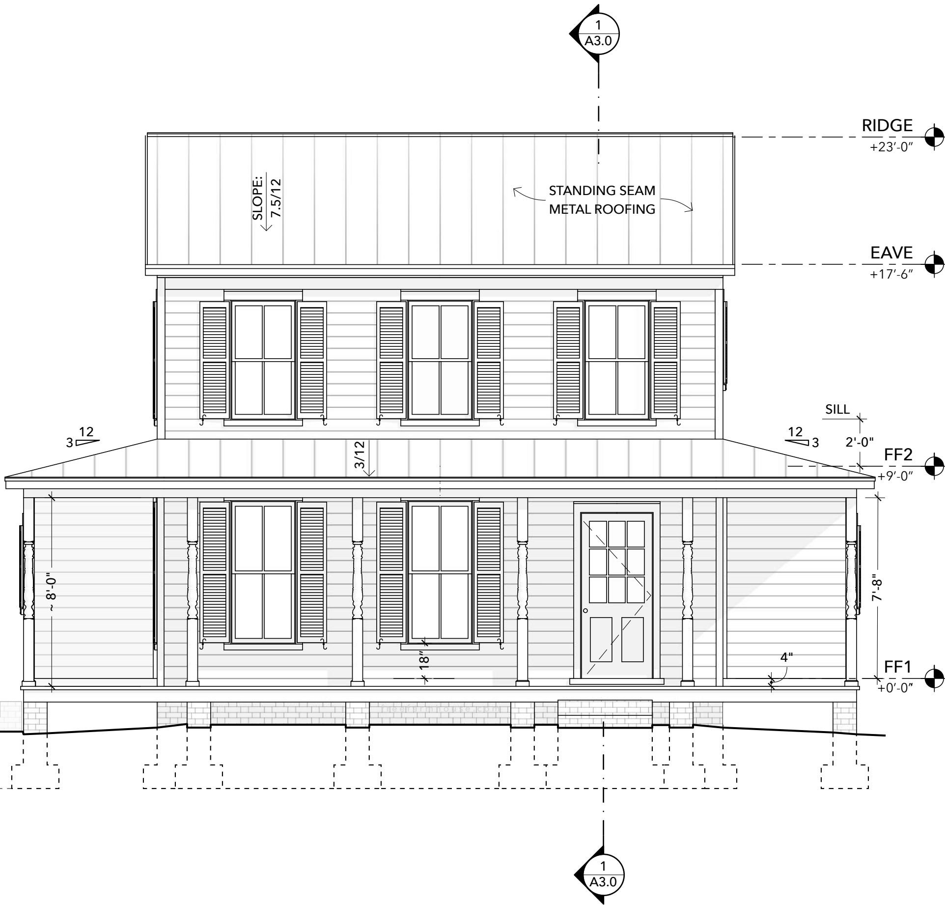
2 SOUTH ELEVATION (FRONT) SCALE: 1/4" = 1'-0"
