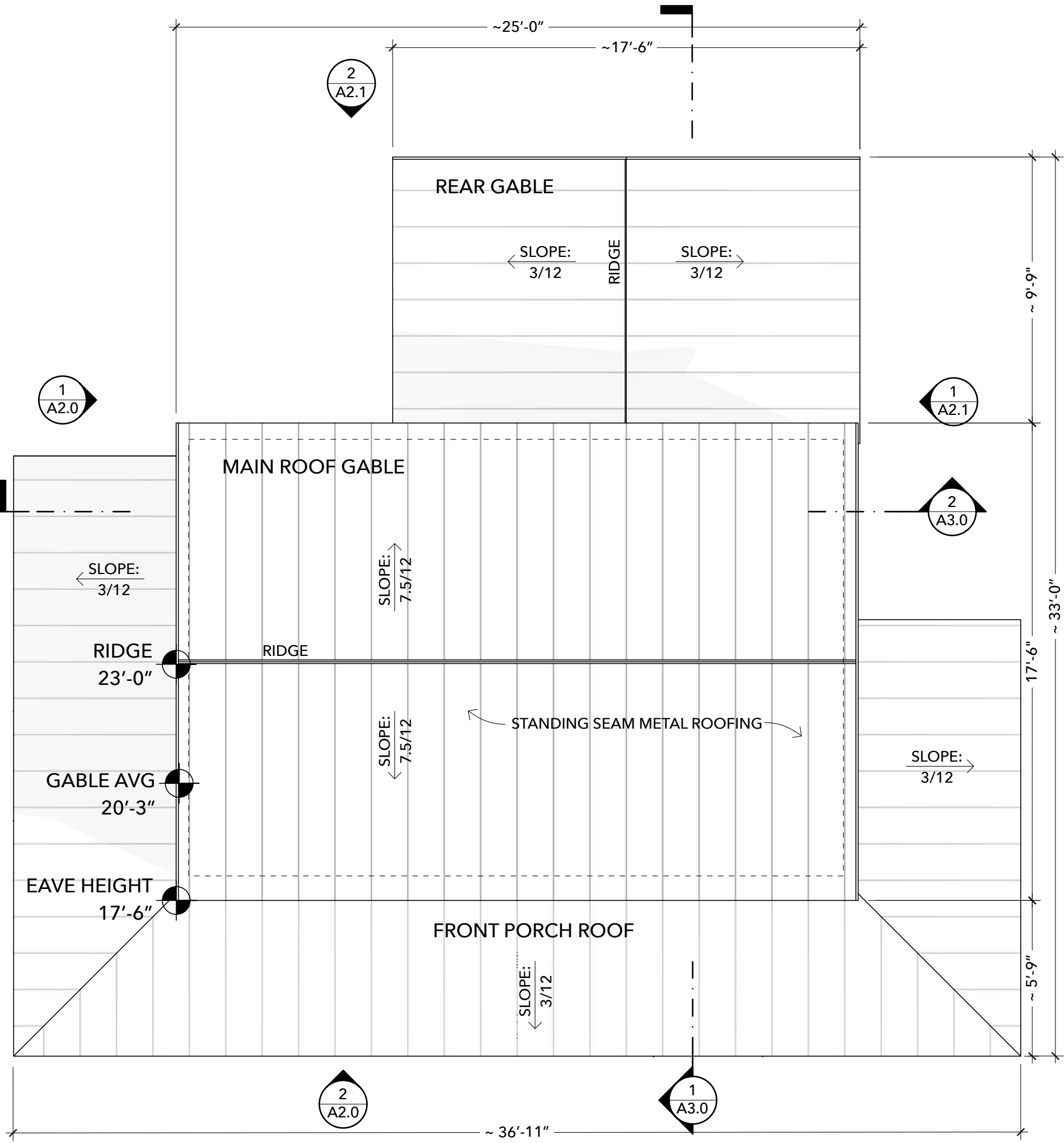
2 ROOF PLAN SCALE: 1/4" = 1'-0"
