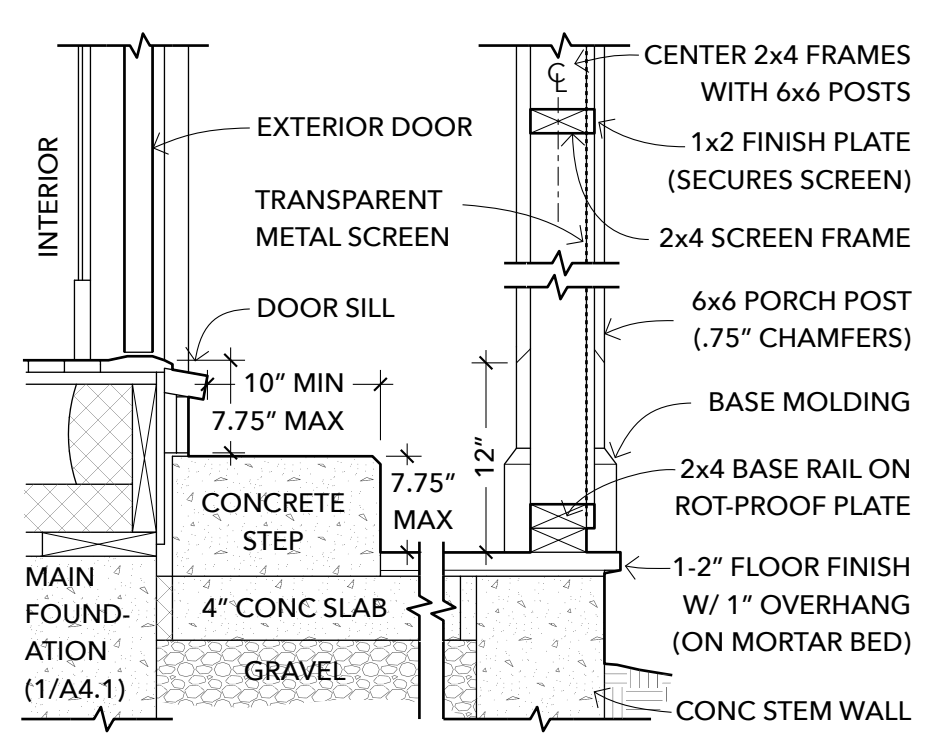
7 SCREEN PORCH @ CONC SLAB SCALE: 1" = 1'-0"
