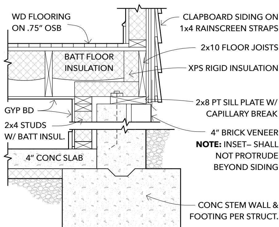
1B FOUNDATION OPT B: BASEMENT SCALE: 1" = 1'-0" OPTION (PORCH NOT SHOWN)
