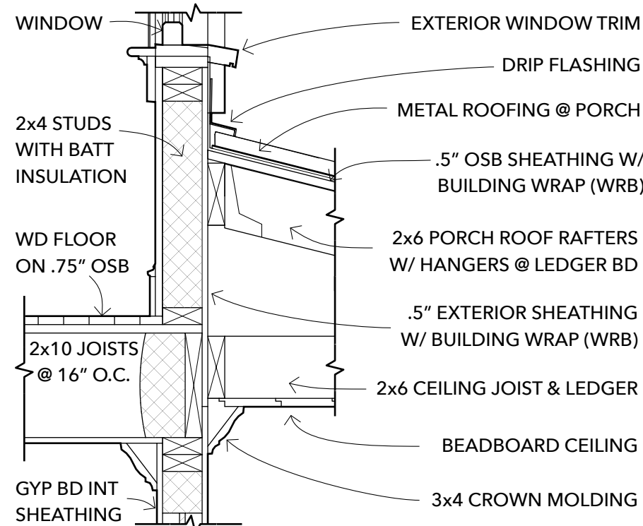
4 PORCH ROOF @ WALL SCALE: 1" = 1'-0"
