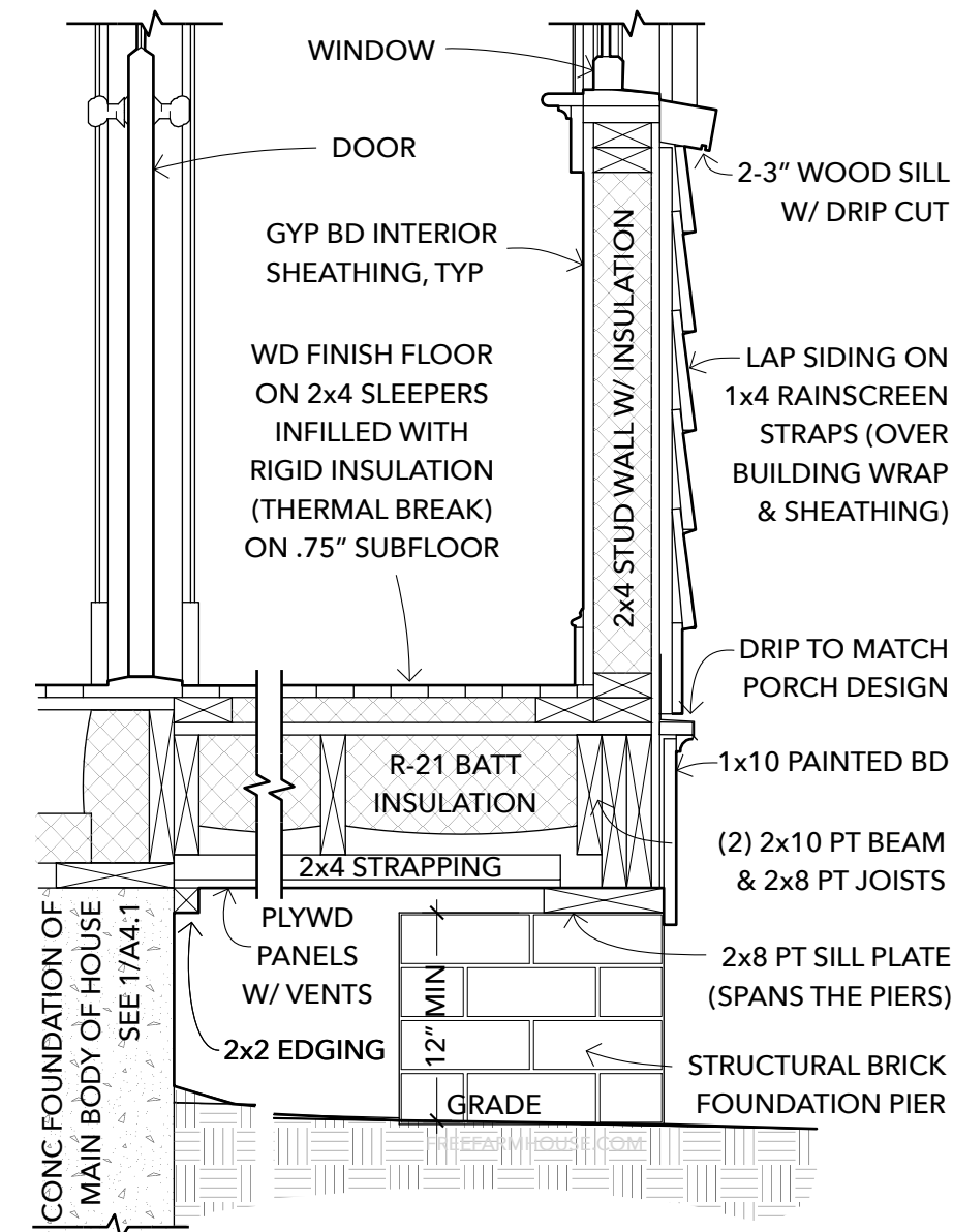
6 INSULATED "PORCH ADDITION" SCALE: 1" = 1'-0" NOTE: TO BE BUILT IN PHASE 1
