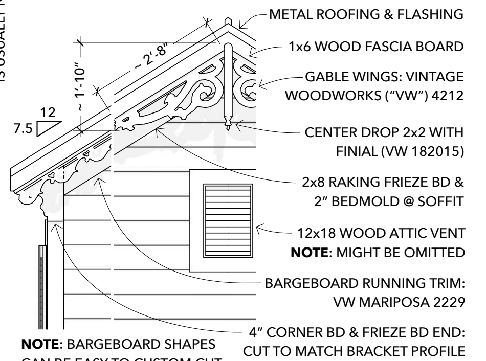
8 GABLE ORNAMENT (OPTION) SCALE: 1/2" = 1'-0" GINGERBREAD DECORATIONS
