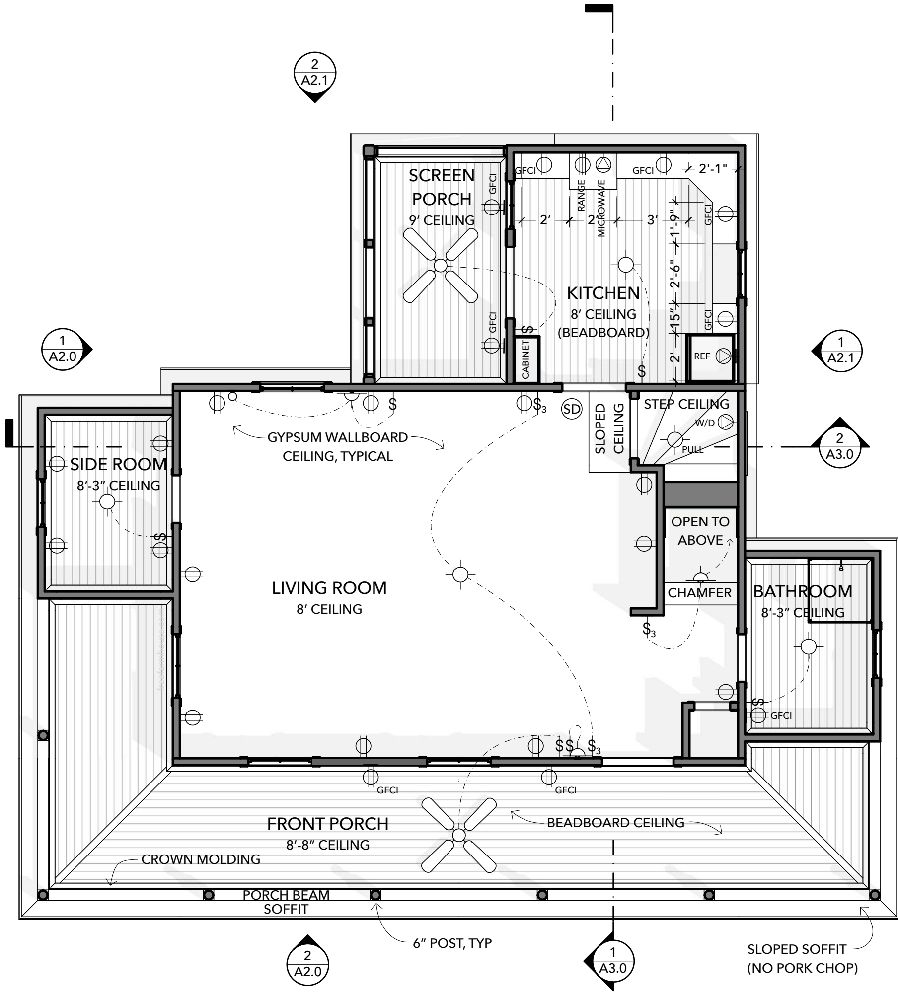
2 DOWNSTAIRS CEILING & ELECTRICAL PLAN SCALE: 1/4" = 1'-0"
